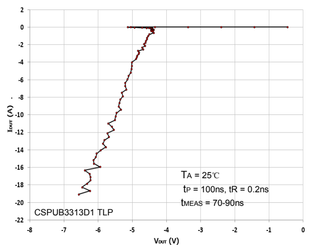
TLP Characteristic (Negative Pulse)
